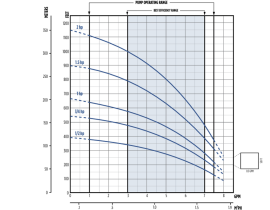
3200 SERIES PUMPS - 5 GPM
