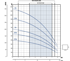
3200 SERIES PUMPS - 5 GPM
